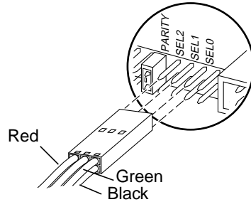
FIGURE 3-3 A Typical SCSI ID Cable Connection
