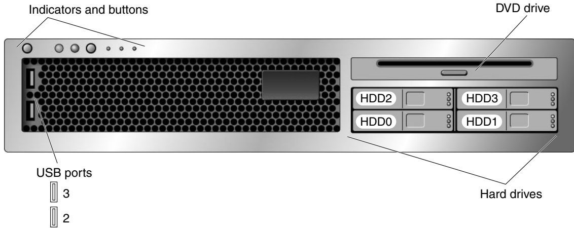
FIGURE 3 Sun SPARC Enterprise T2000 Server Front Panel
