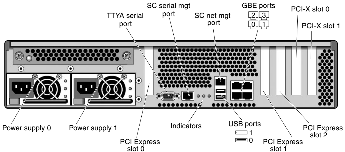
FIGURE 4 Sun SPARC Enterprise T2000 Server Rear Panel
