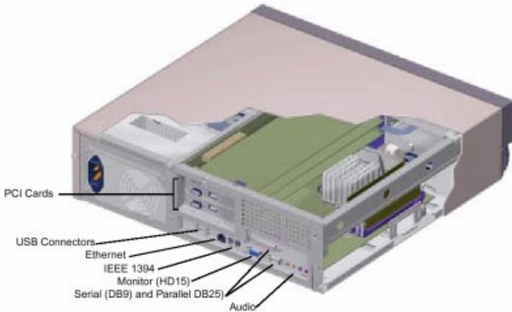
Figure 3. Rear view of Sun Blade 150 workstation, showing connectors
